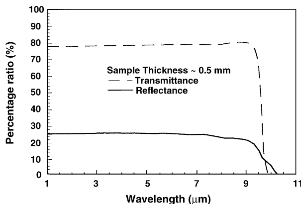
Fig. 3. Optical properties of a 500 μm thick YSZ sample (Source: Dr. Zhuomin Zhang, unpublished work).
